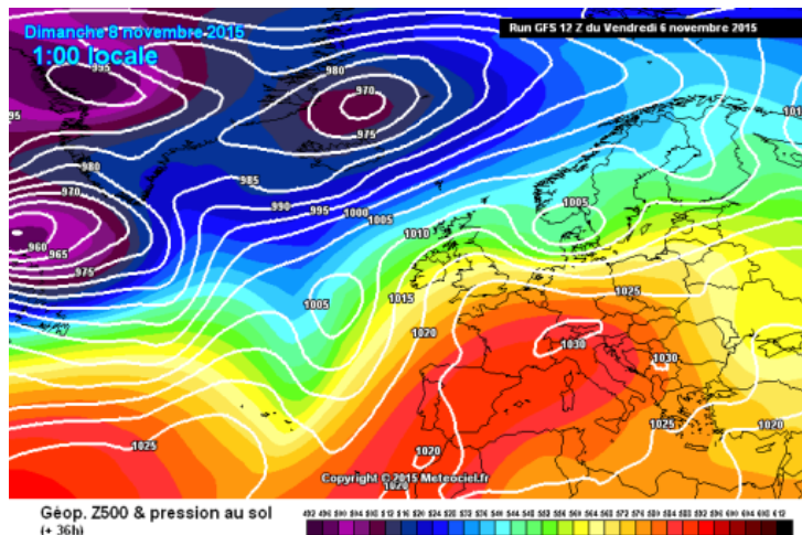
A "warm blooded high" is currently dominating the Alps - Image: meteociel.com
